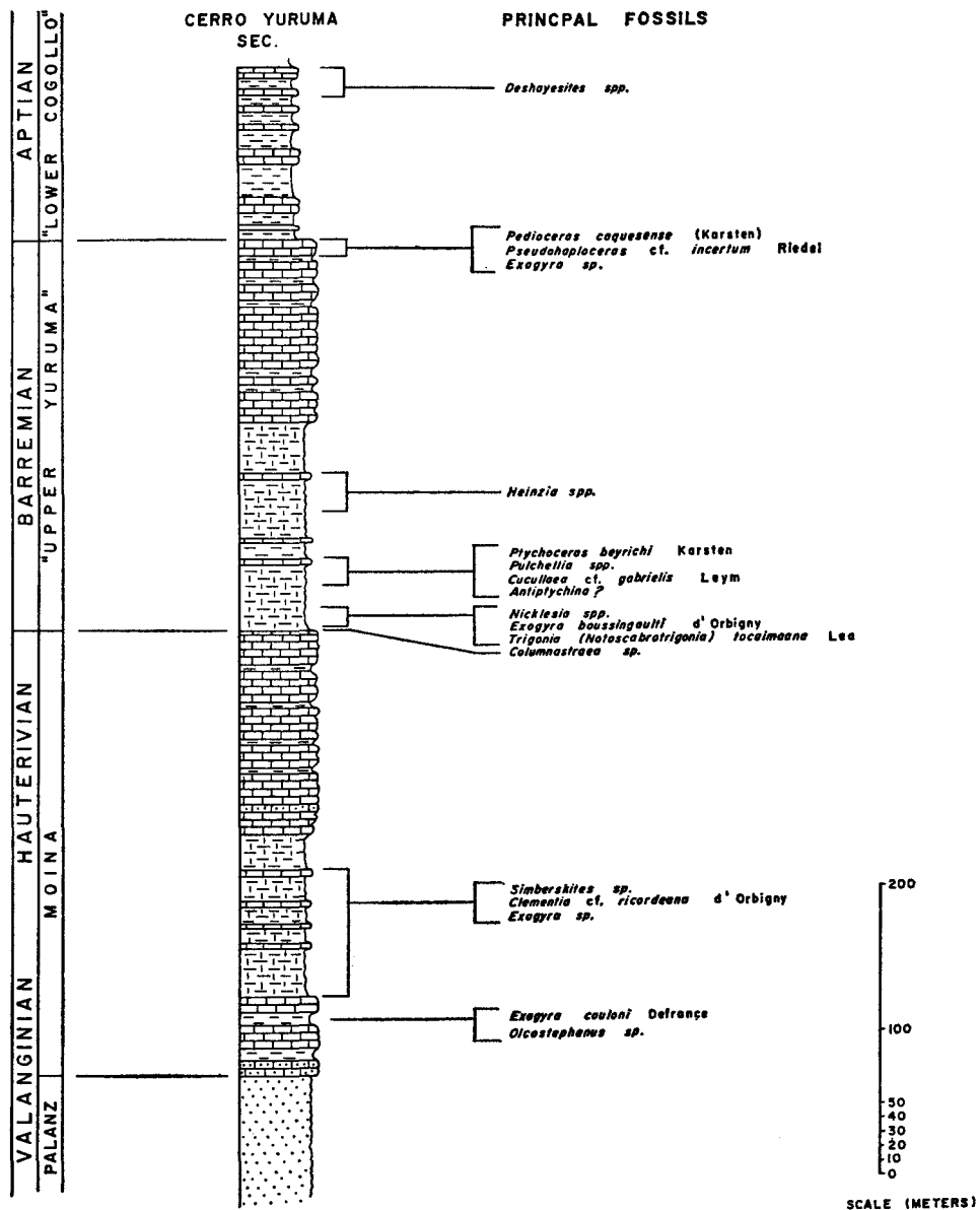
FIG. - 6 FAUNAL ZONES YURUMA GROUP
