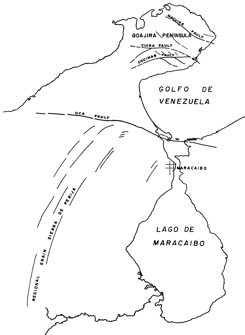
FIG.-II REGIONAL TECTONIC FRAMEWORK WESTERN VENEZUELA
