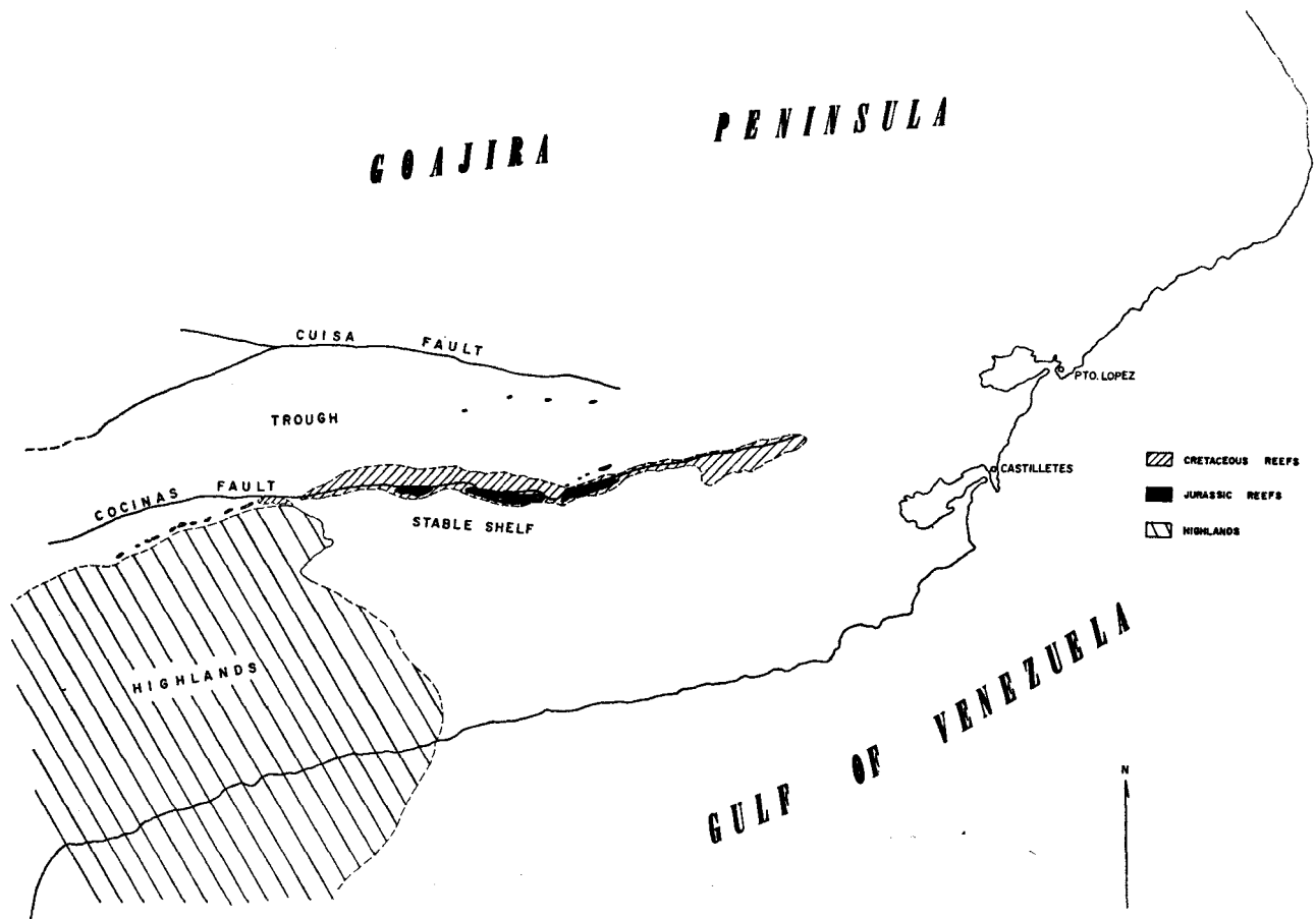
FIG.-5 JURASSIC AND CRETACEOUS REEF DEVELOPMENT
