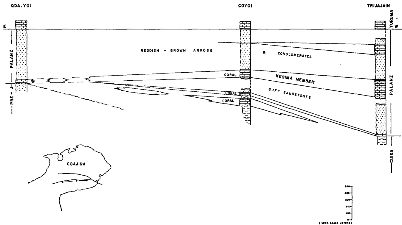
FIG.-4 STRATIGRAPHIC DIAGRAM OF PALANZ FORMATION
