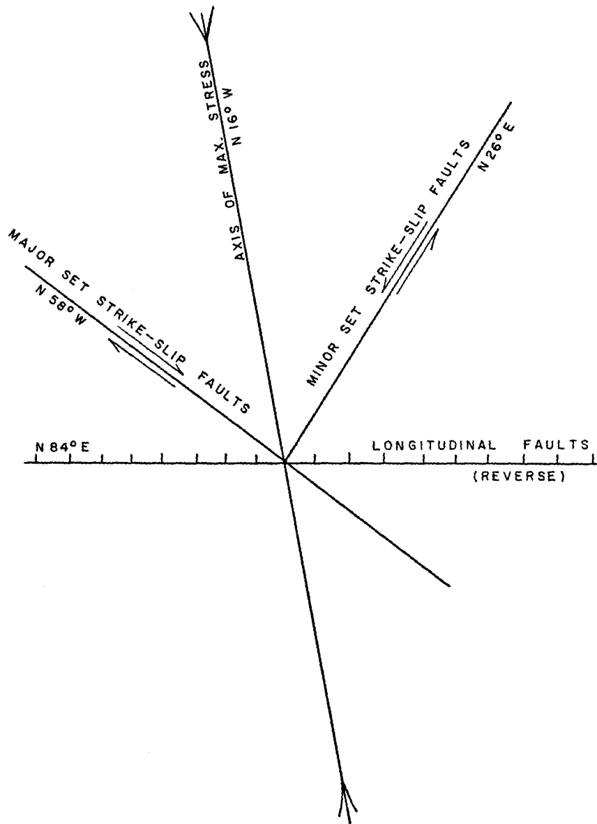
FIG.—16 RELATION OF AXIS OF MAXIMUM COMPRESSION TO AVERAGE TRENDS OF FAULT SETS IN PART OF COCINAS TROUGH
