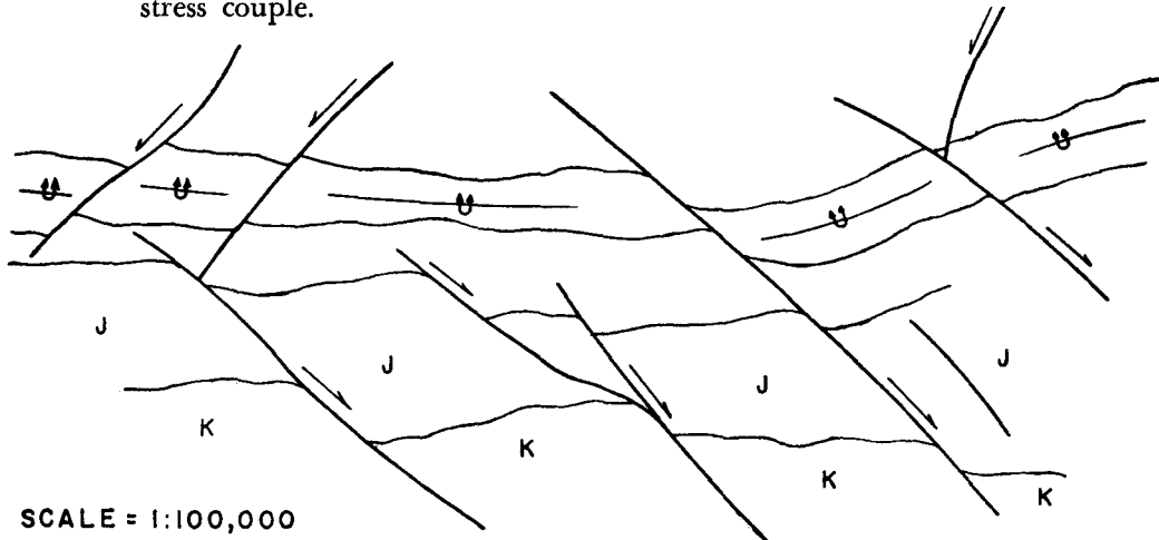
FIG.—14 ILLUSTRATIONS OF STRIKE-SLIP FAULT PATTERN DUE TO COMPRESSION. (Reduced 10% from original art work.)
