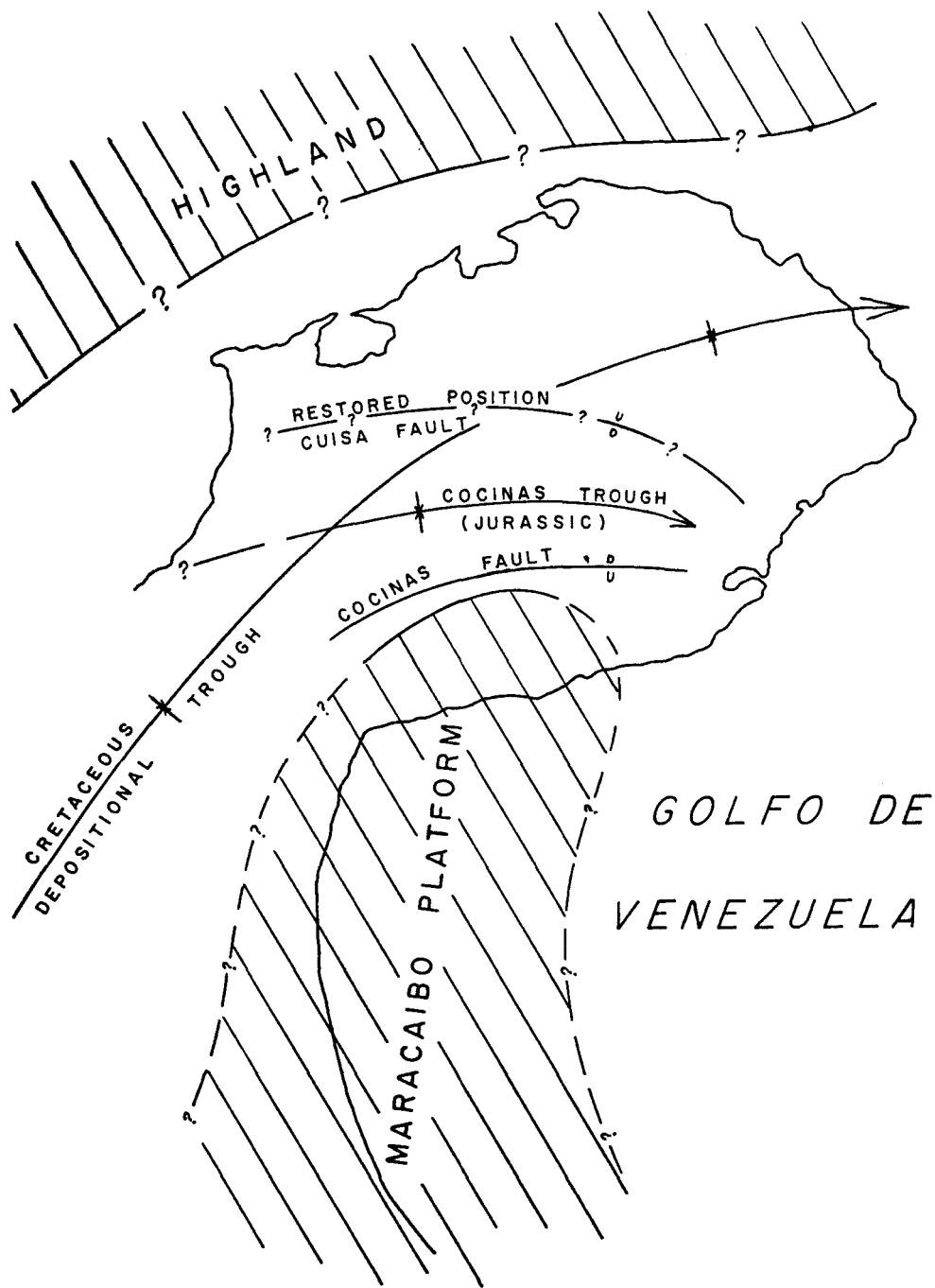
FIG.—12 MESOZOIC TECTONIC FRAMEWORK OF GOAJIRA
